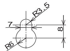
Mounting hole 1 (1 : 1)
