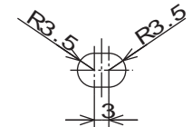
Mounting hole 1 (1 : 1)
