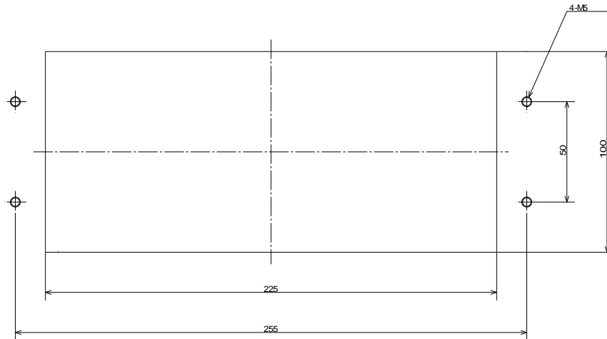
Panel cutout dimensions
